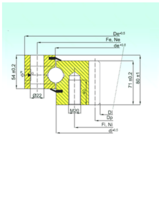
ZB1.25.1455.200-1SPTN Bearing 2D drawings and 3D CAD models
